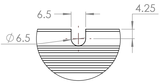
DETAIL A 4x SCALE 1 : 1
